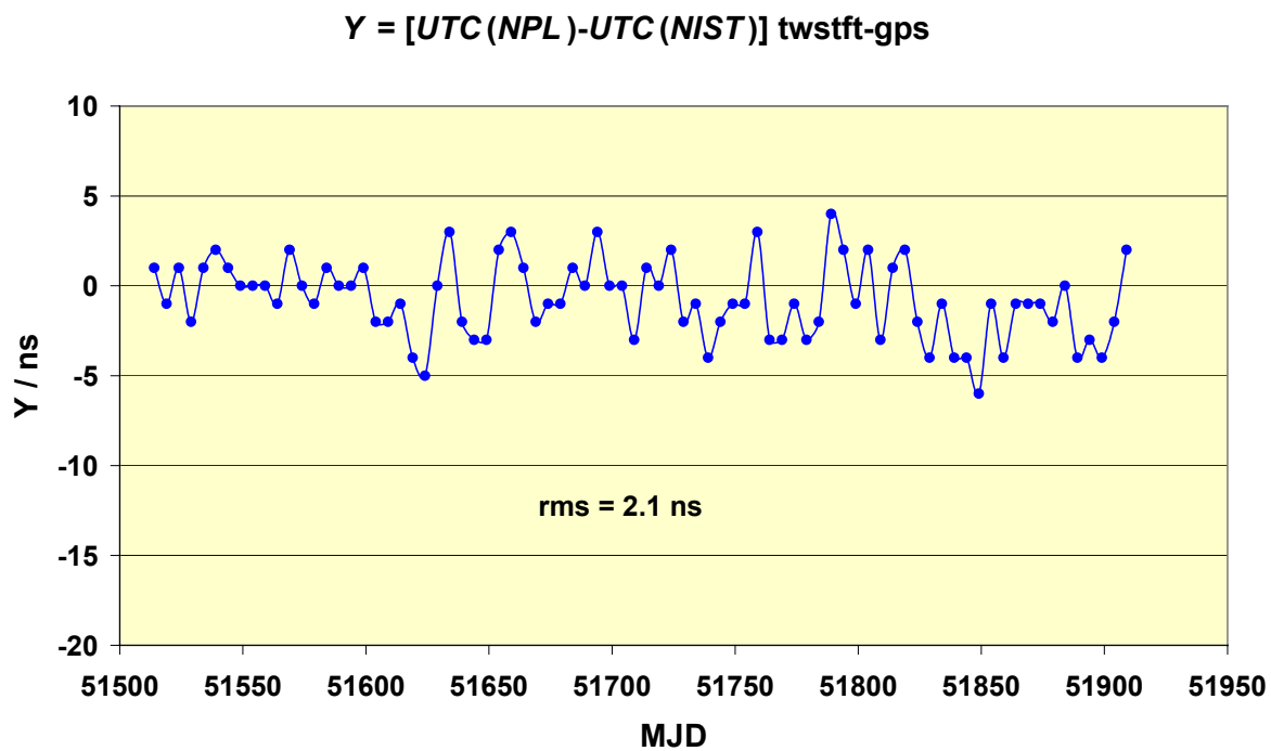
Figure 5. Differences between TWSTFT and GPS C/A-code common-view for NPL/NIST link
