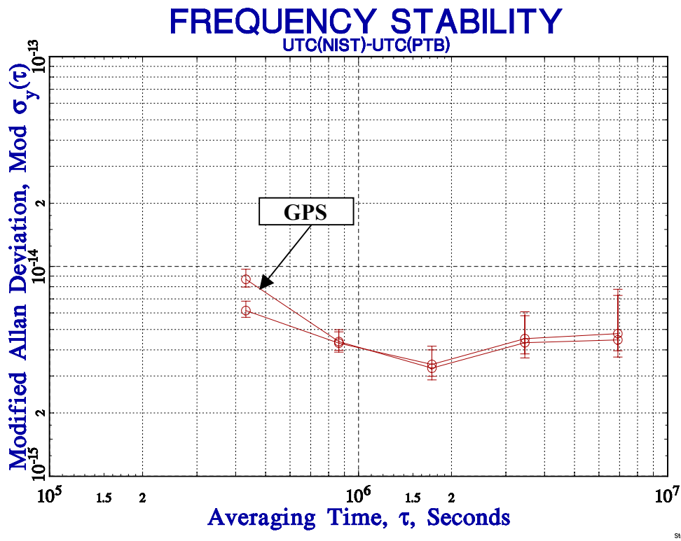
Figure 1. Frequency stability of [UTC(NIST) - UTC(PTB)] by GPS CV and by TWSTFT.
