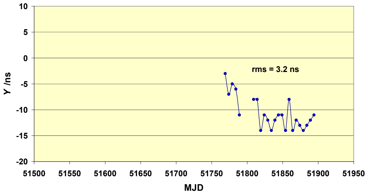
Figure 2b. Differences between TWSTFT (NPL station 02) and GPS C/A-code common-view for USNO/NPL link.
