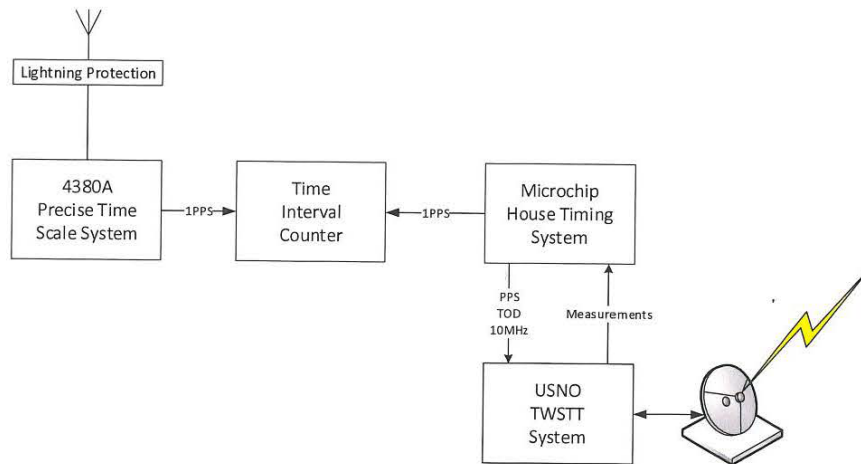
System Calibration Test Configuration
