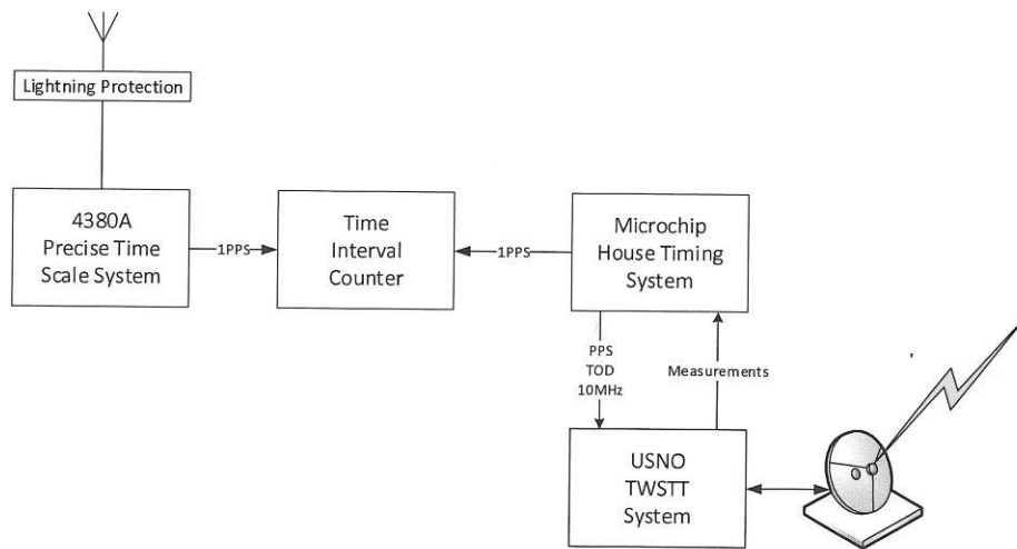
System Calibration Test Configuration
