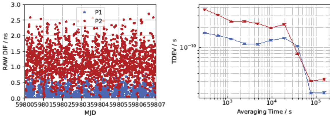
Figure B-7 Left: Raw code differences between T and ES09 for GPS signals, \Delta P1 (blue) and \Delta P2 (red) Right: TDEV of the raw code differences between T and ES09 for GPS signals.
