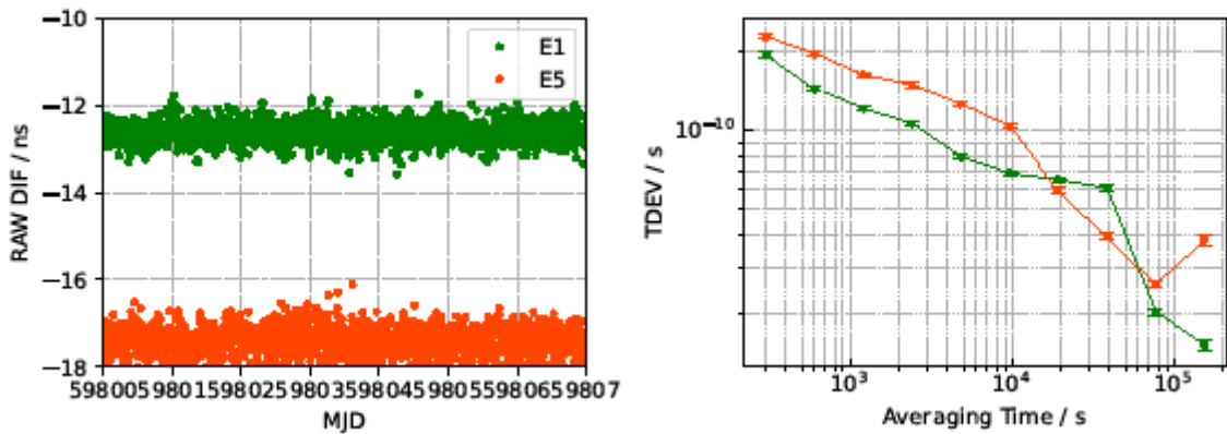
Figure B-6 Left: Raw code differences between T and ES08 for Galileo signals, \Delta E1 (green) and \Delta E5a (orange) Right: TDEV of the raw code differences between T and ES08 for Galileo signals.
