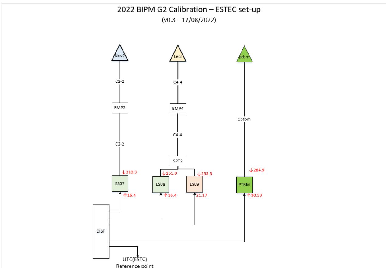
Figure 3-4 PPS signal distribution at ESTEC to the receivers
