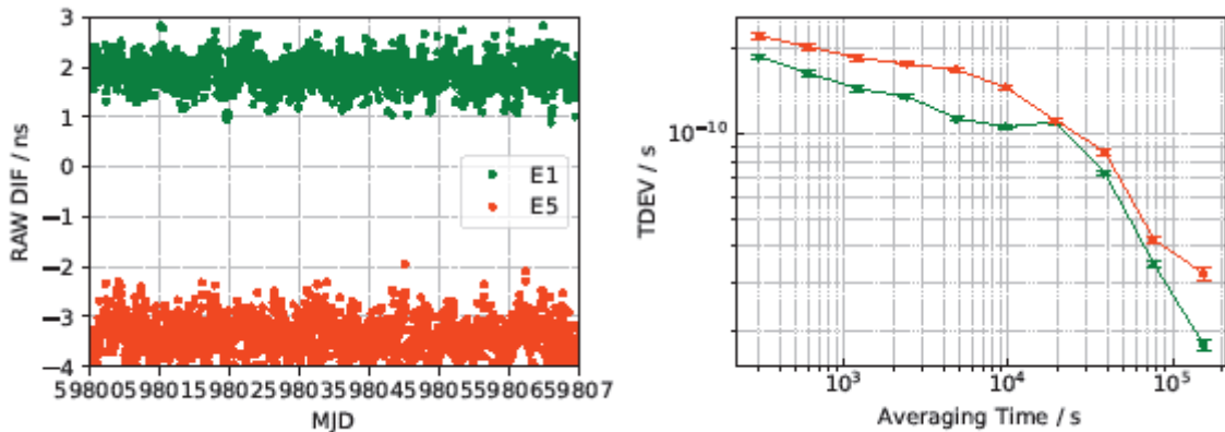
Figure B-8 Left: Raw code differences between T and ES08 for Galileo signals, \Delta E1 (green) and \Delta E5a (orange) Right: TDEV of the raw code differences between T and ES09 for Galileo signals.
