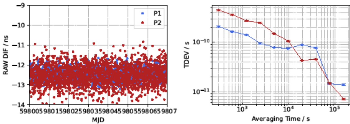
Figure B-5 Left: Left: Raw code differences between T and ES08 for GPS signals, \Delta P1 (blue) and \Delta P2 (red) Right: TDEV of the raw code differences between T and ES08 for GPS signals.
