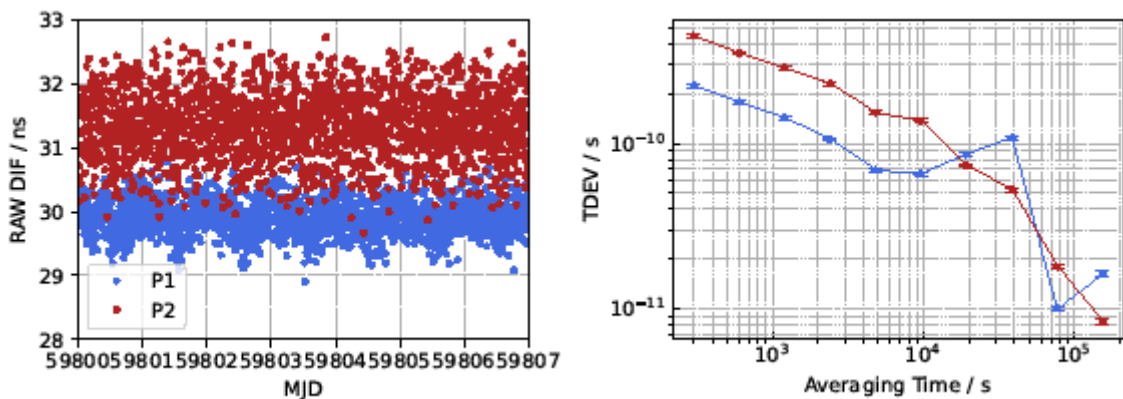
Figure B-3 Left: Left: Raw code differences between T and ES07 for GPS signals, \Delta P1 (blue) and \Delta P2 (red) Right: TDEV of the raw code differences between T and ES07 for GPS signals.
