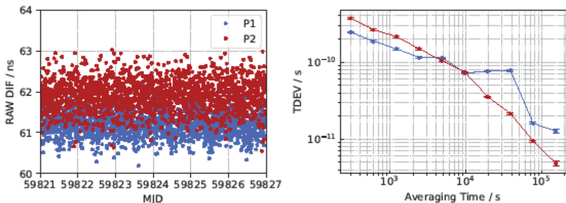
Figure B-9 Left: Raw code differences between T and G for GPS signals during CC2, \Delta P1 (blue) and \Delta P2 (red) Right: TDEV of the raw code differences between T and G for GPS signals during CC2.
