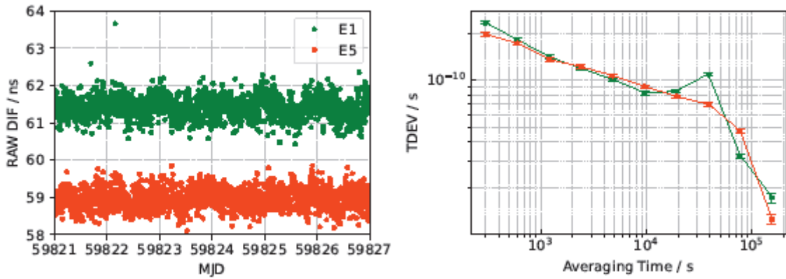
Figure B-10 Left: Raw code differences between T and G for Galileo signals during CC2, \Delta E1 (green) and \Delta E5a (orange) Right: TDEV of the raw code differences between T and G for Galileo signals during CC2.
