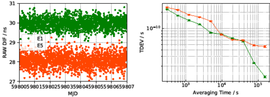
Figure B-4 Left: Raw code differences between T and ES07 for Galileo signals, \Delta E1 (green) and \Delta E5a (orange) Right: TDEV of the raw code differences between T and ES07 for Galileo signals.
