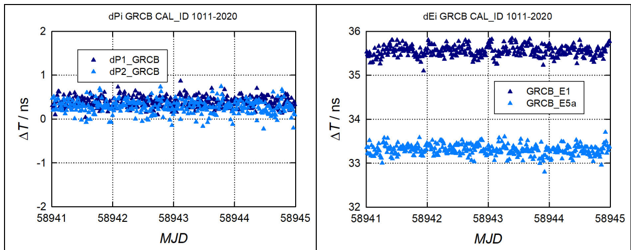
Figure 6-7. Corrections to INT DLY in GRCB, reference PTBM; left: GPS \Delta P1 (dark) and \Delta P2 (light), right: Galileo, \Delta E1 (dark) and \Delta E5a (light).
