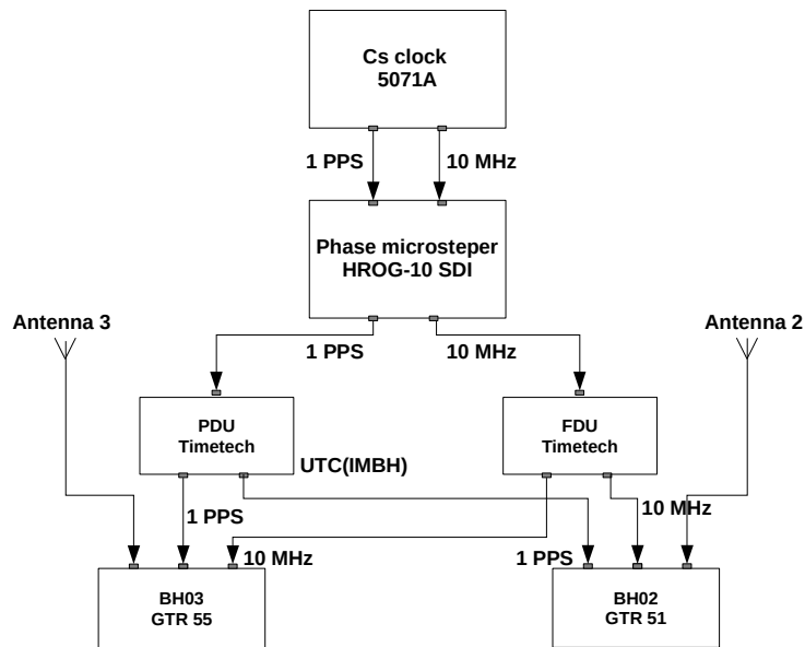
Figure 1: Diagram of experiment setup
