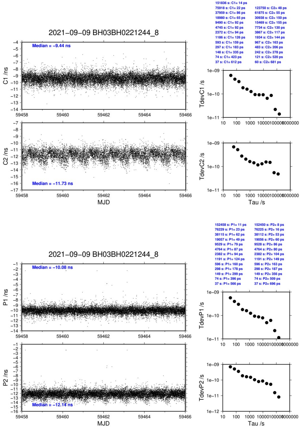
Figure 3: Plots of RAW data and TDEV analysis
