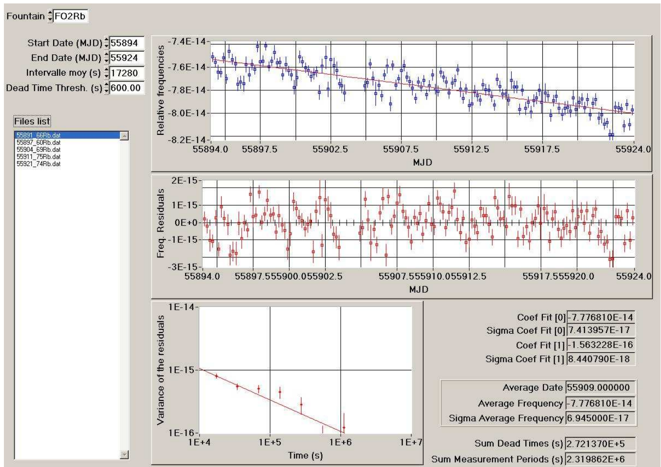
Figure 1: Processing of the data HMaser_{140\ 0890} -FO2Rb for the period MJD 55894-55924
