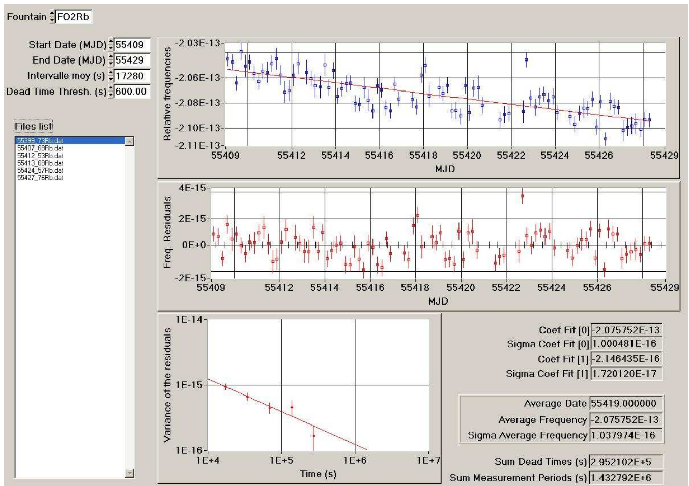
Figure 1: Processing of the data HMaser_{140\ 0890} -FO2Rb for the period MJD 55409-55429
