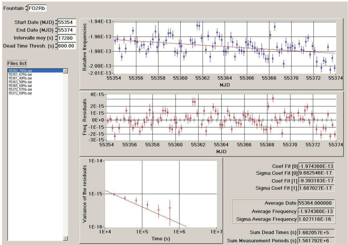
Figure 1: Processing of the data HMaser_{140\ 0890} -F02Rb for the period MJD 55354-55374
