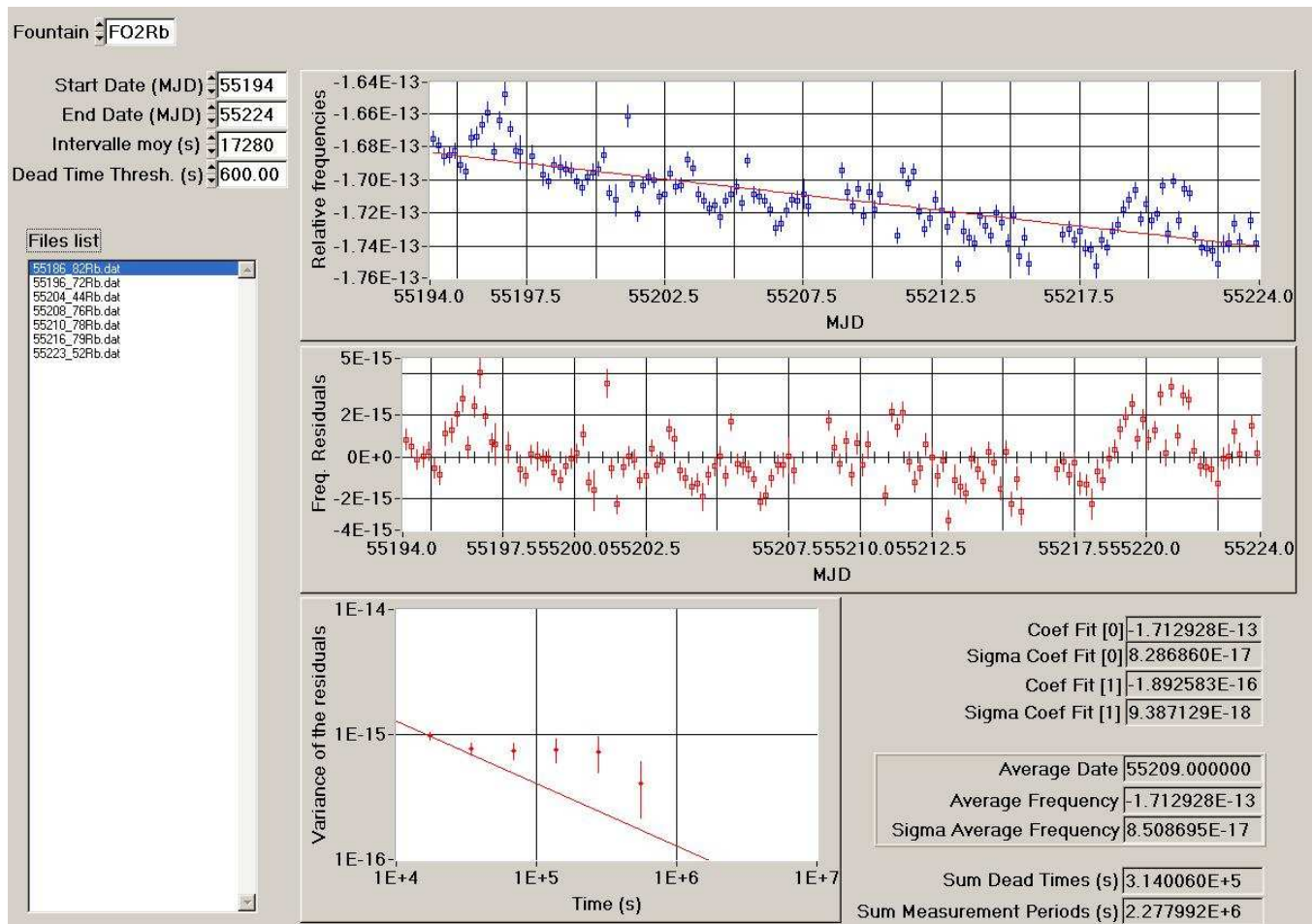
Figure 1: Processing of the data HMaser_{140\ 0890} -FO2Rb for the period MJD 55194-55224
