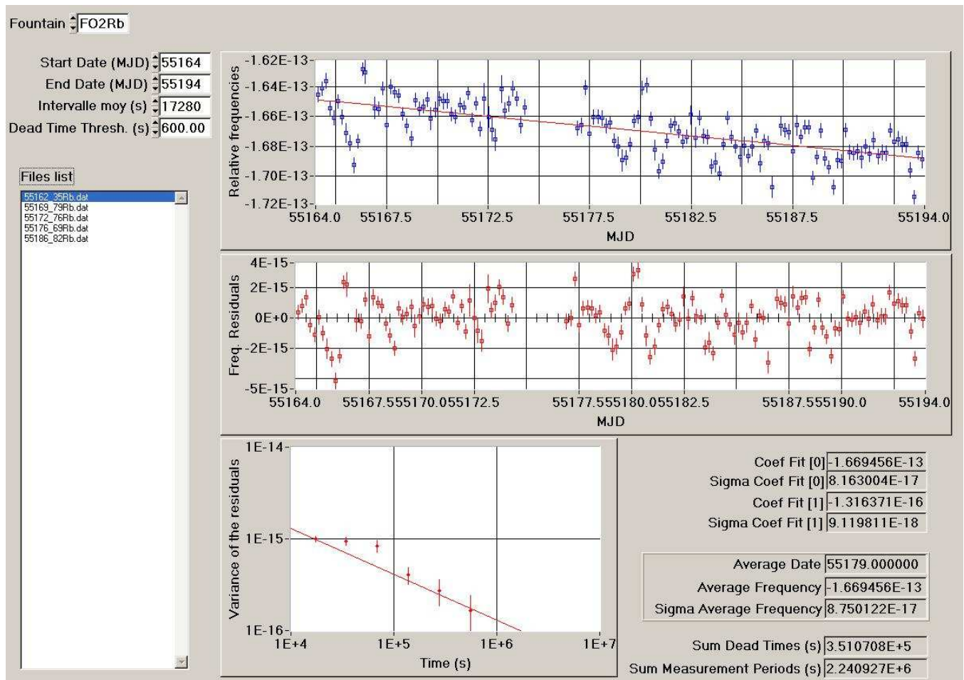
Figure 1: Processing of the data HMaser_{140\ 0890} -FO2Rb for the period MJD 55164-55194
