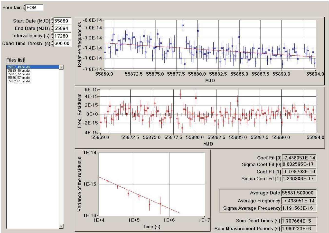
Figure 1: Data processing for the period MJD 55869-55894
