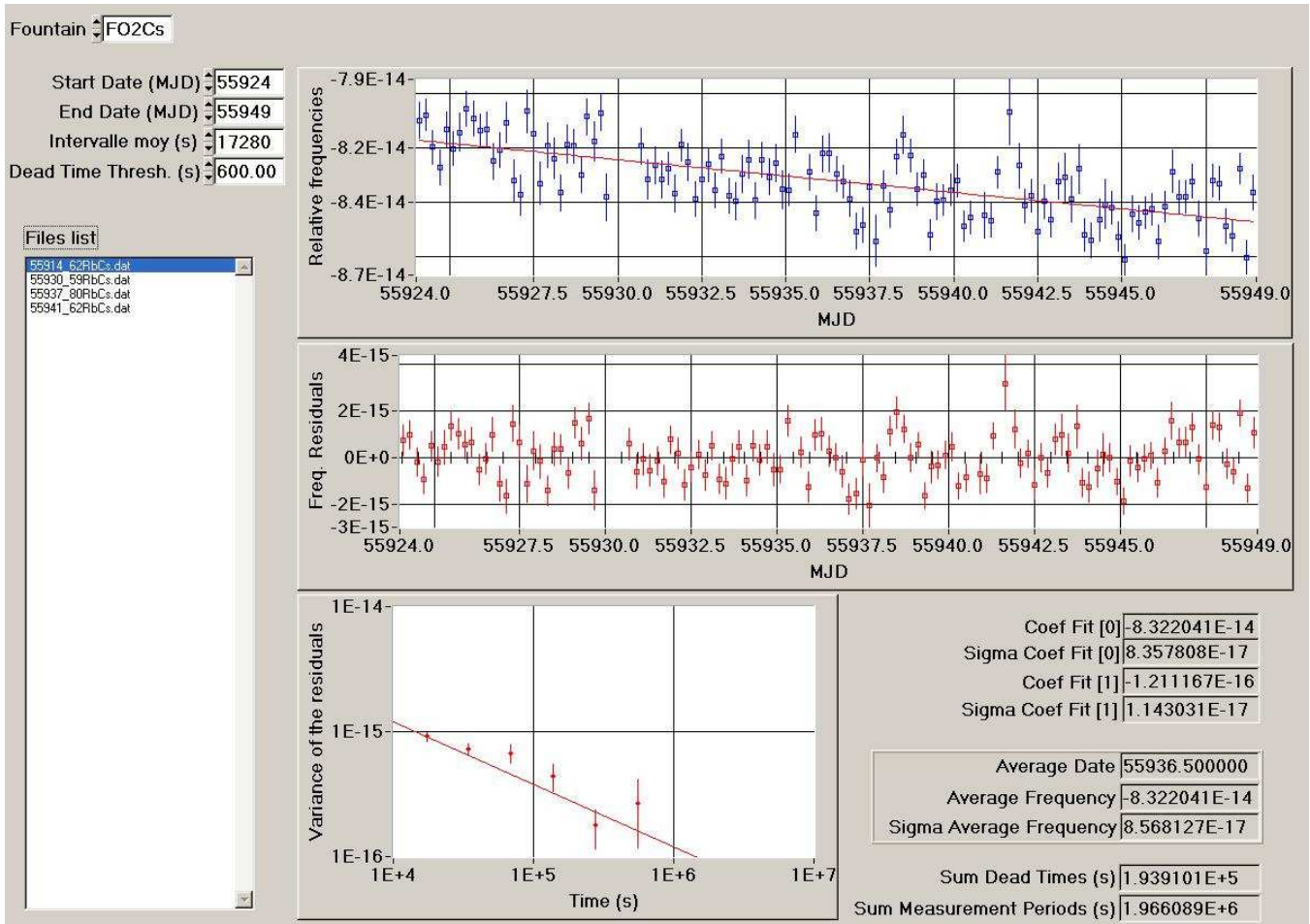
Figure 1: Processing of the data HMaser_{140\ 0890-FO2} for the period MJD 55924-55949
