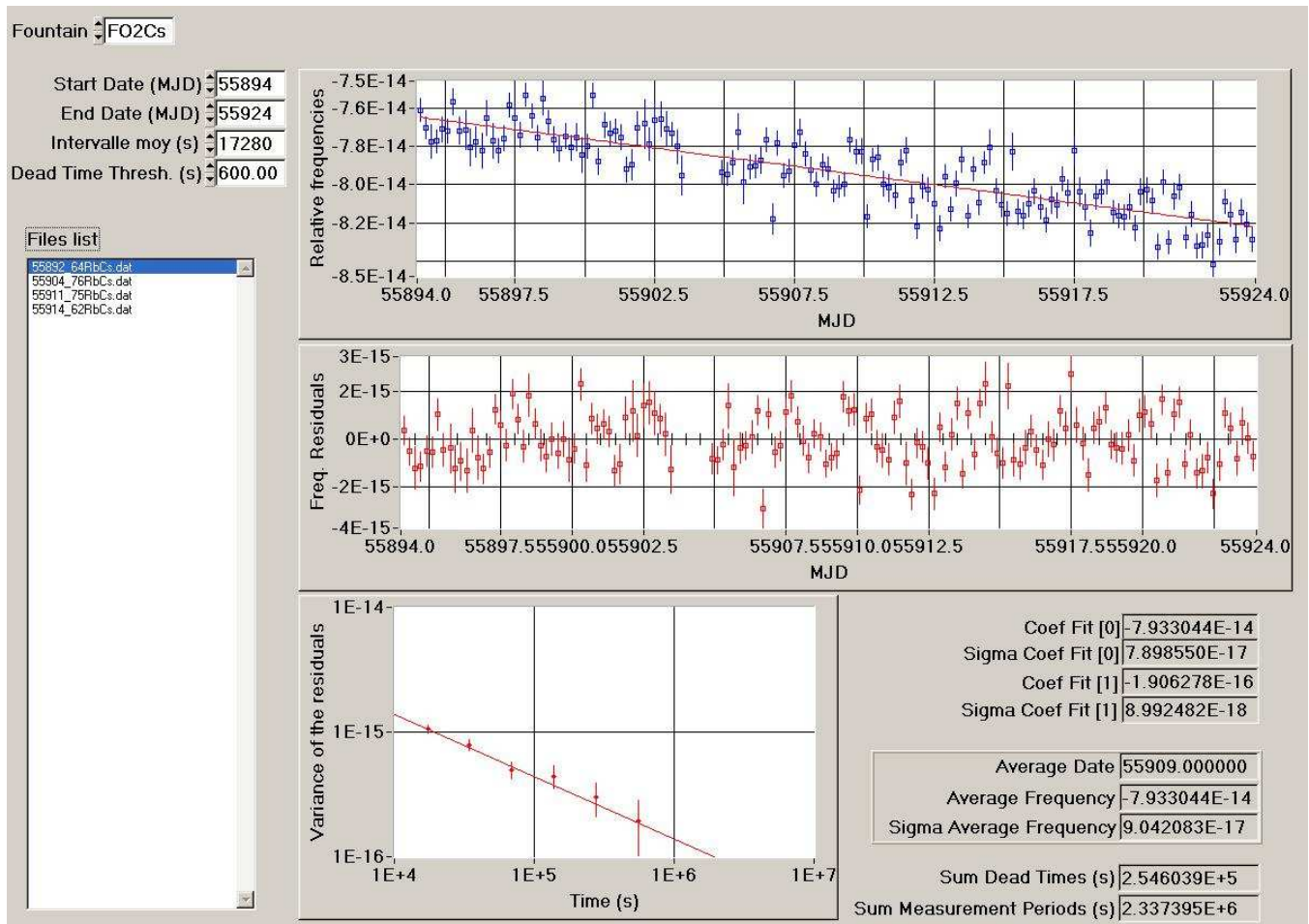
Figure 1: Processing of the data HMaser_{140\ 0890-FO2} for the period MJD 55894-55924
