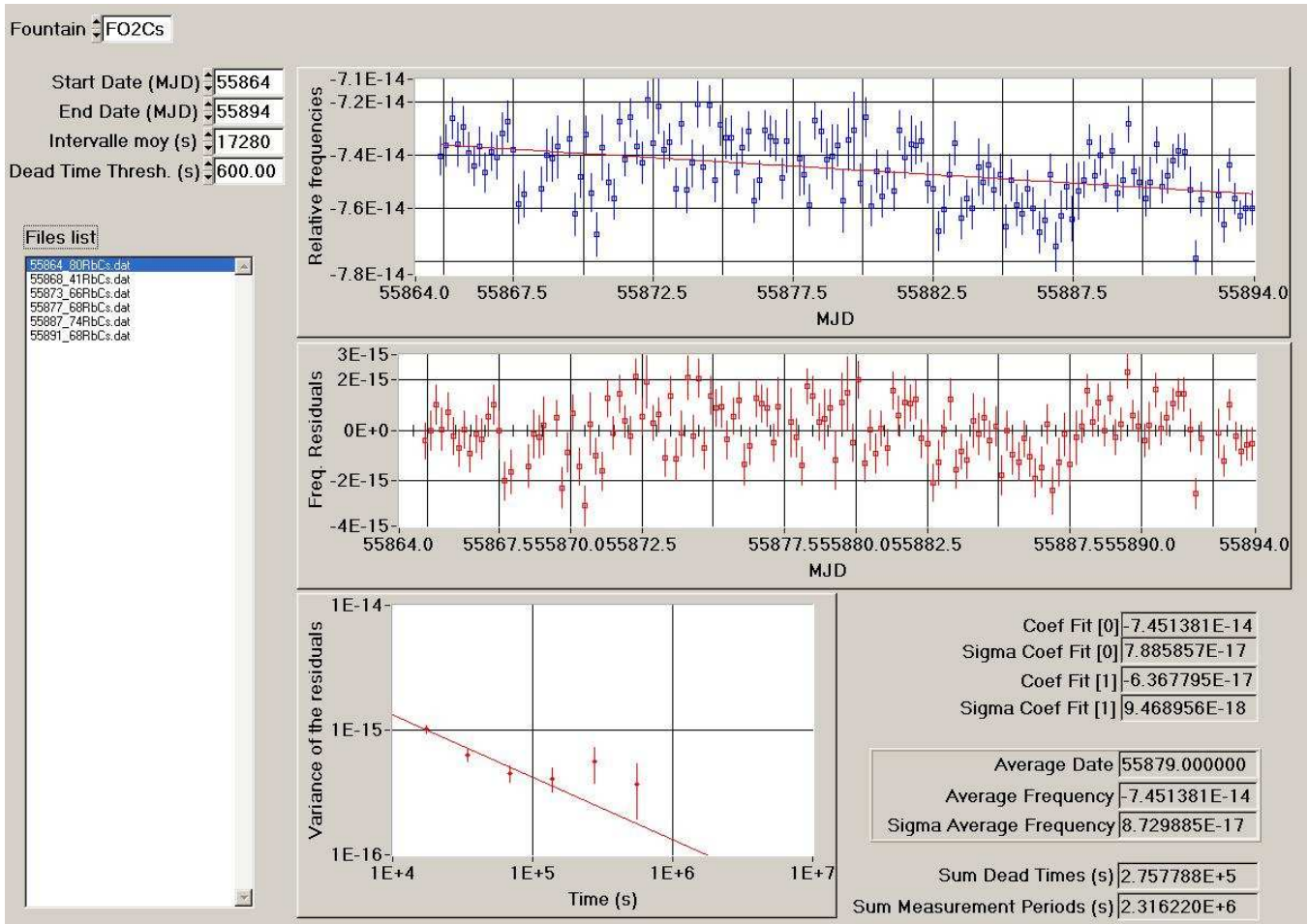
Figure 1: Processing of the data HMaser_{140\ 0890-FO2} for the period MJD 55864-55894
