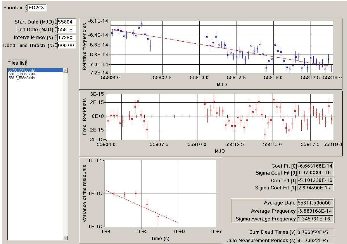
Figure 1: Processing of the data HMaser_{140\ 0890-FO2} for the period MJD 55804-55819
