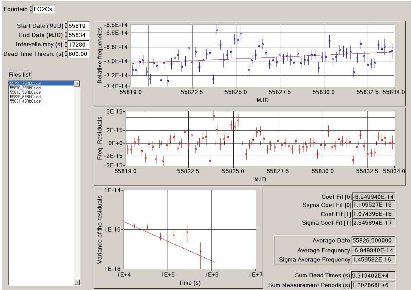
Figure 2: Processing of the data HMaser_{140\ 0890-FO2} for the period MJD 55819-55834
