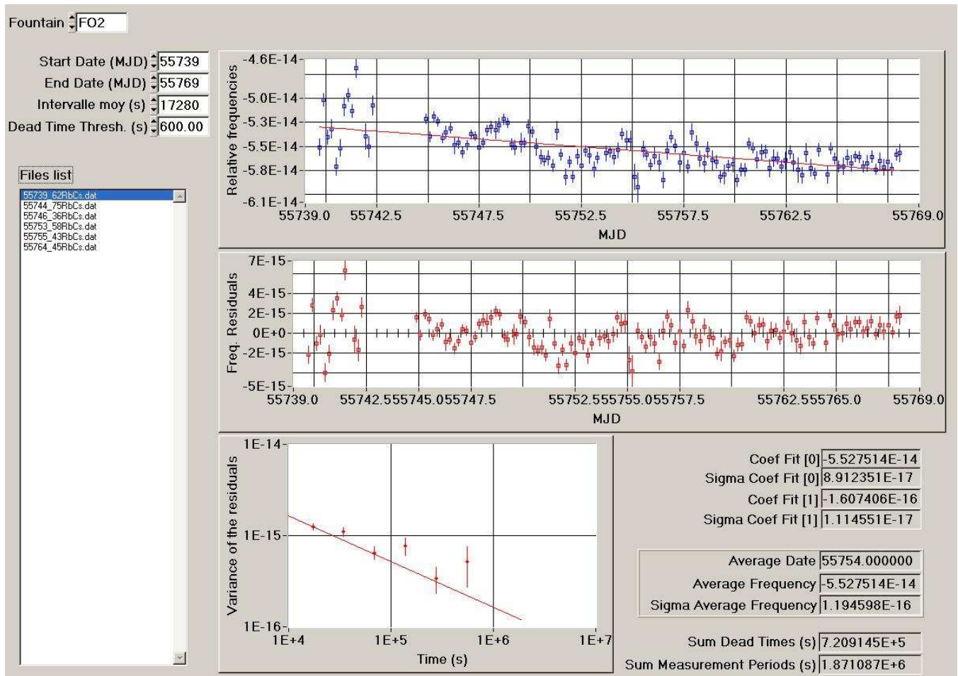
Figure 1: Processing of the data HMaser 140 0890 -FO2 for the period MJD 55739-55769
