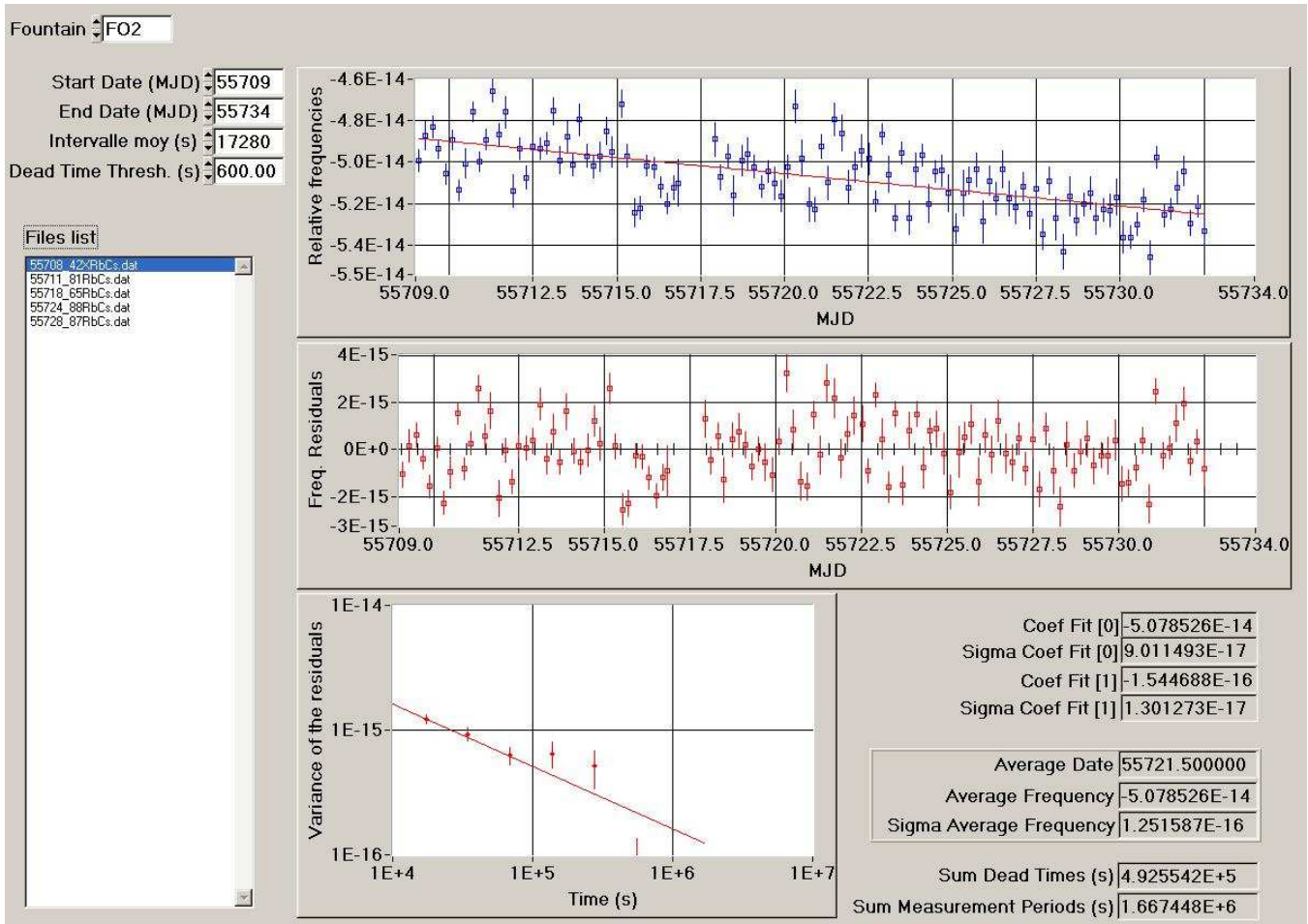
Figure 1: Processing of the data HMaser_{140\ 0890} -FO2 for the period MJD 55709-55734
