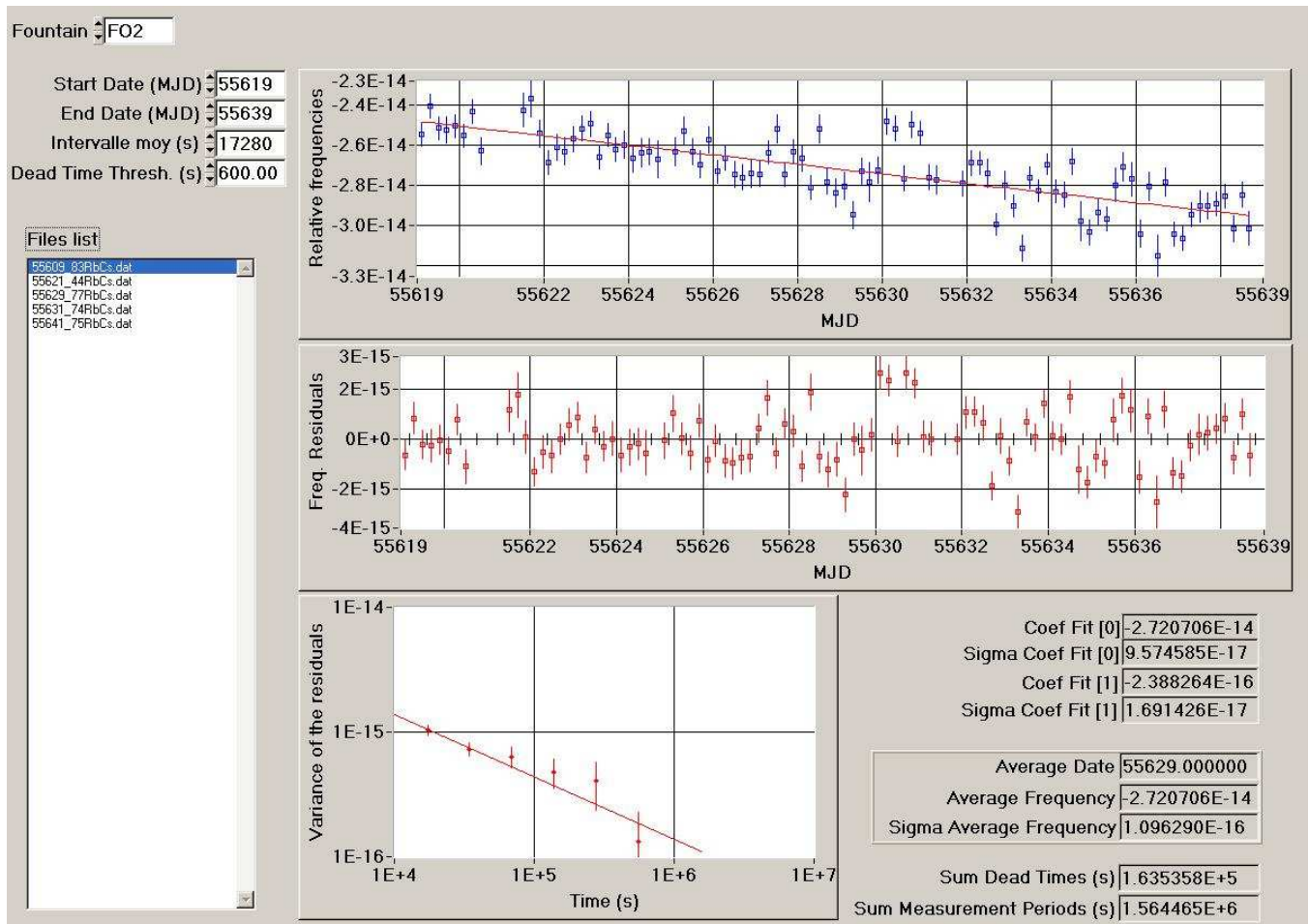
Figure 1: Processing of the data HMaser_{140\ 0890-FO2} for the period MJD 55619-55639
