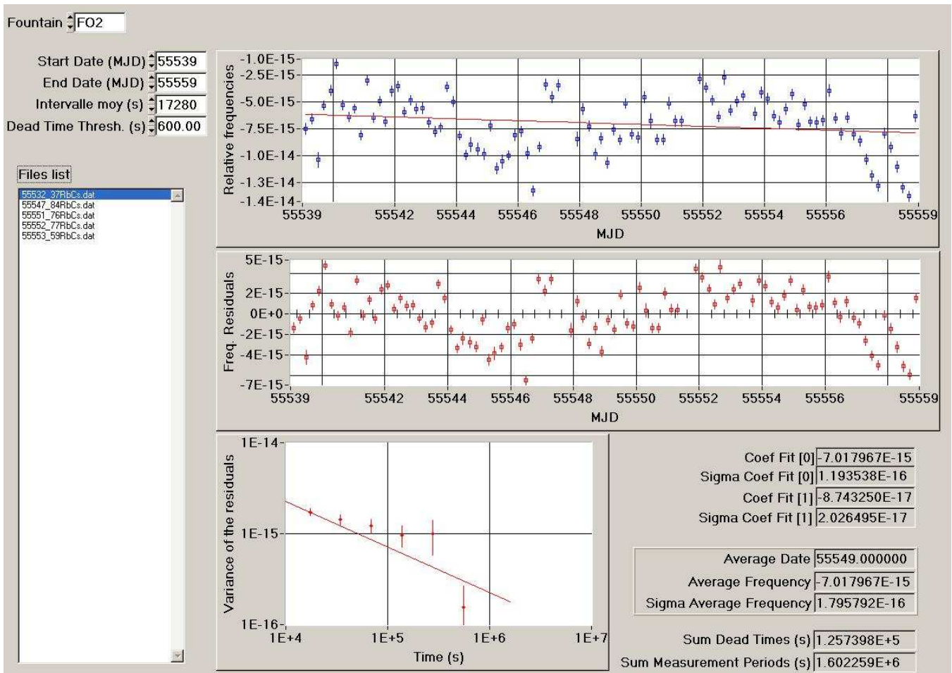
Figure 1: Processing of the data HMaser_{140\ 0816} -FO2 for the period MJD 55539-55559
