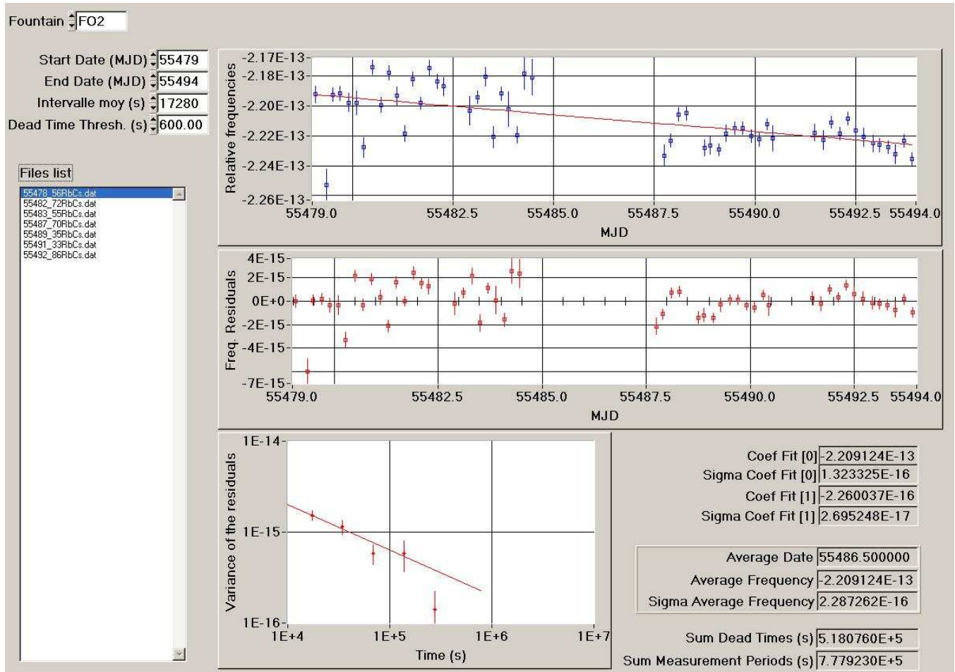
Figure 1: Processing of the data HMaser_{140\ 0890-FO2} for the period MJD 55479-55494
