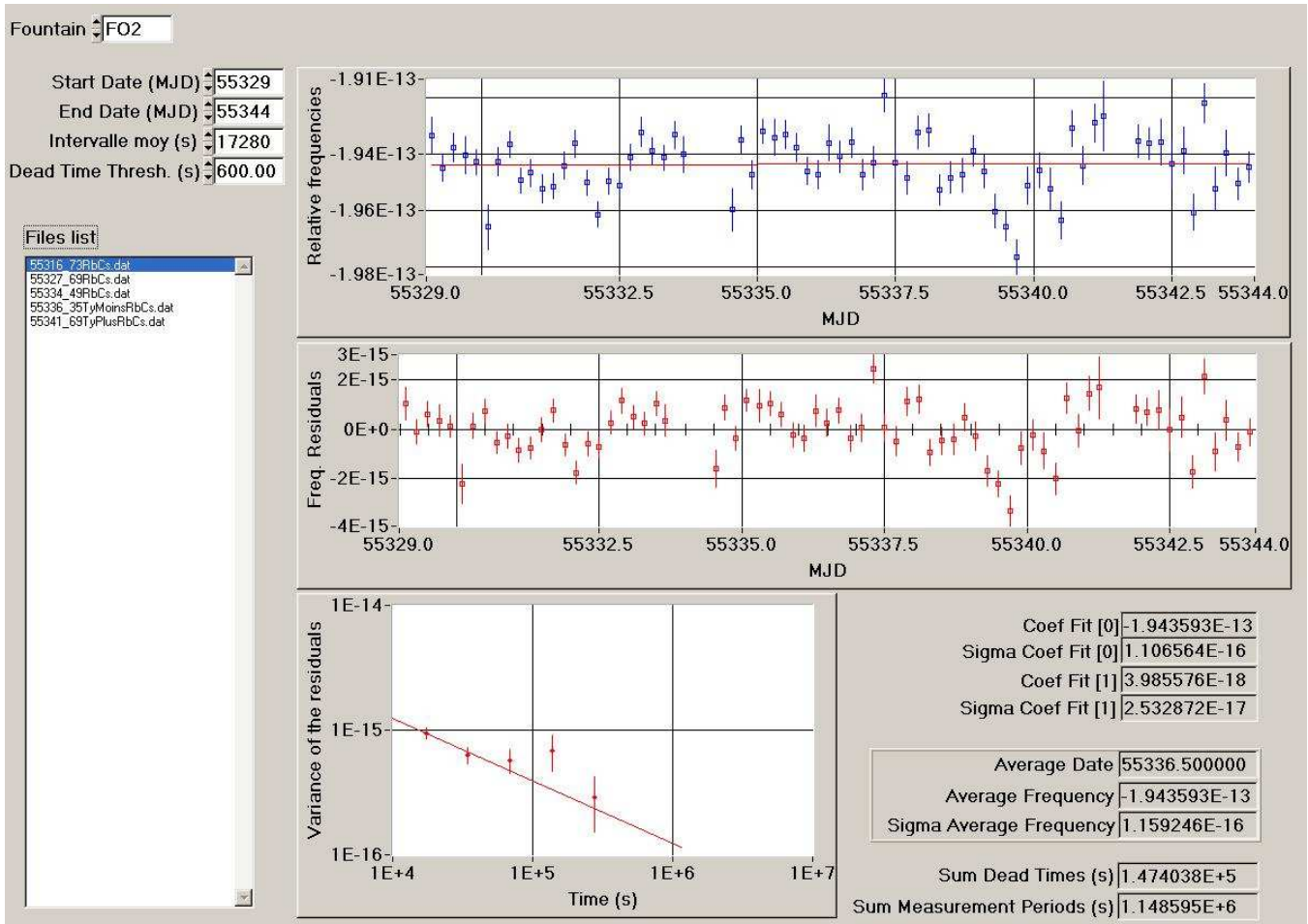
Figure 1: Processing of the data HMaser_{140\ 0890-FO2} for the period MJD 55329-55344
