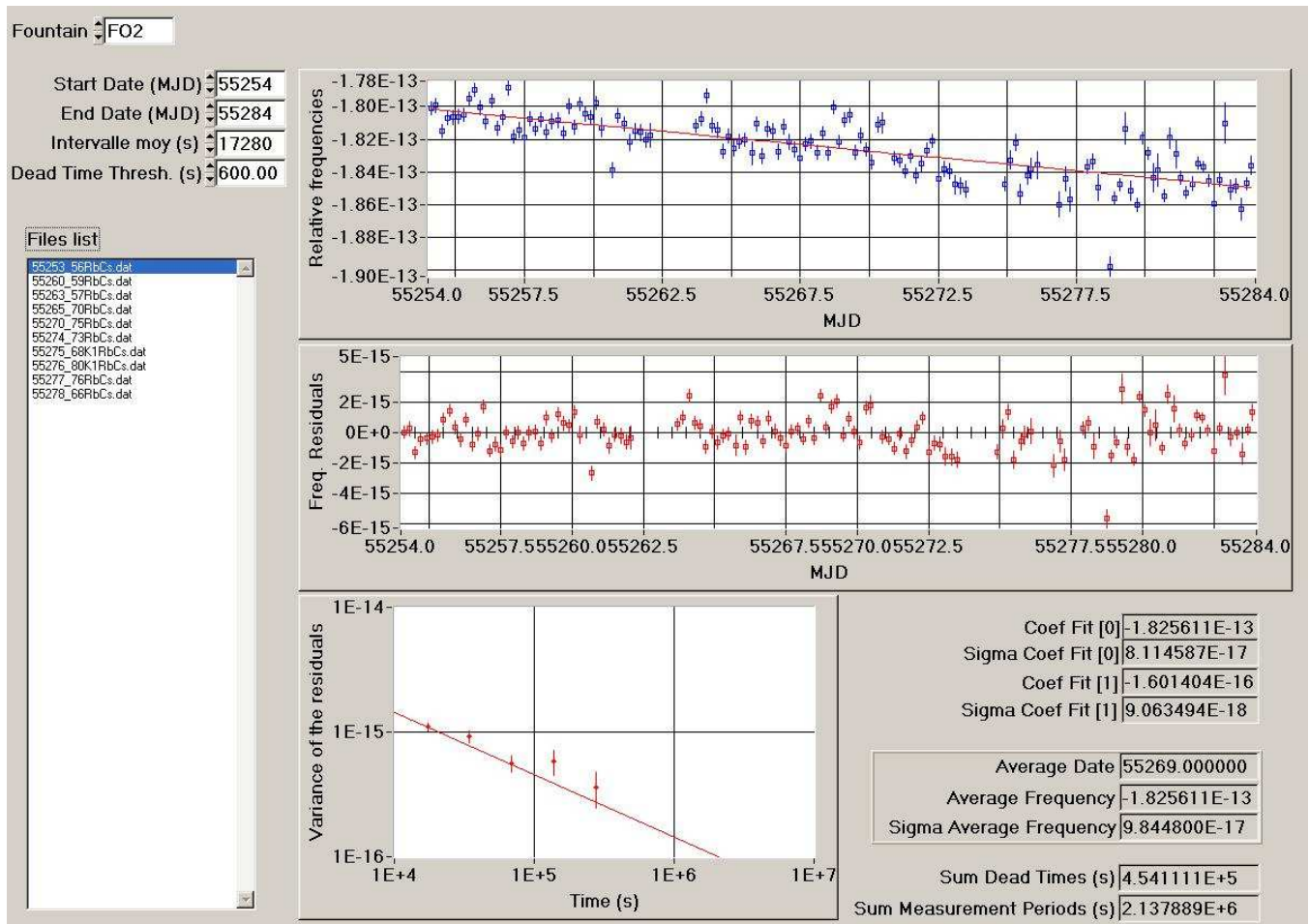
Figure 1: Processing of the data HMaser 140 0890 -FO2 for the period MJD 55254-55284
