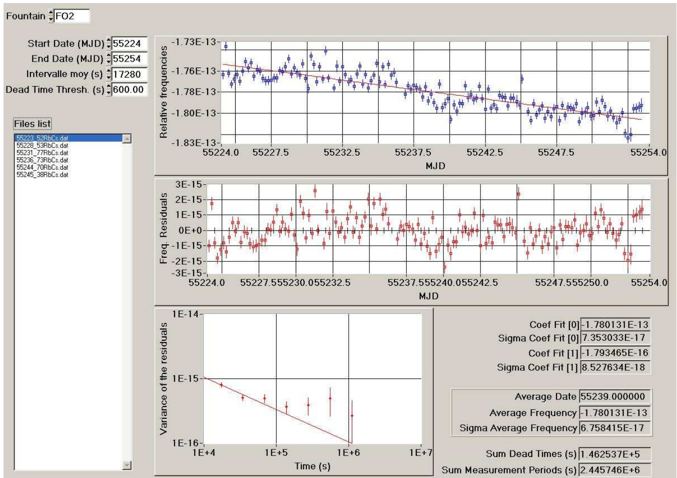
Figure 1: Processing of the data \text{HMaser}_{140\ 0890}\text{-FO2} for the period MJD 55224-55254
