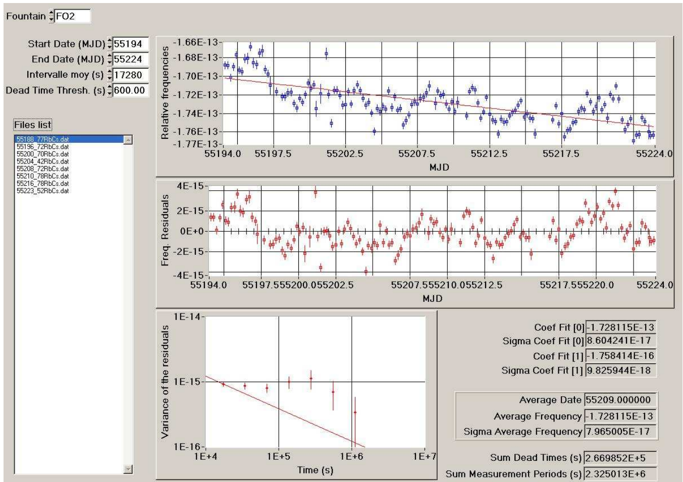
Figure 1: Processing of the data HMaser_{140\ 0890-FO2} for the period MJD 55194-55224
