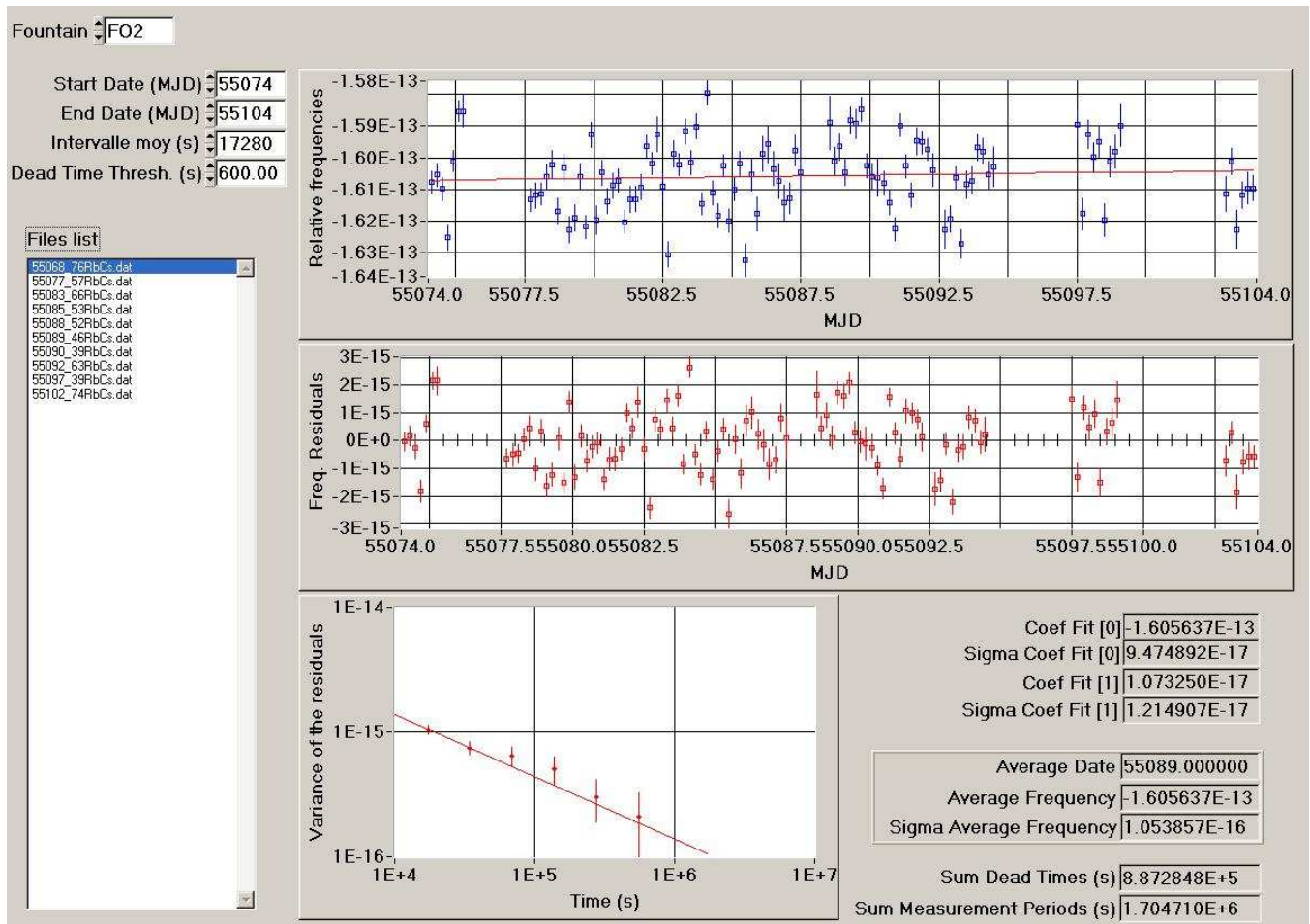
Figure 1: Processing of the data HMaser_{140\ 0890-FO2} for the period MJD 55074-55104
