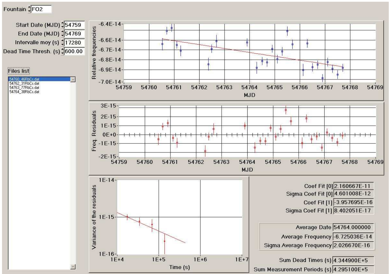
Figure 1: Processing of the data HMaser_{140\ 0890-FO2} for the period MJD 54759-54769
