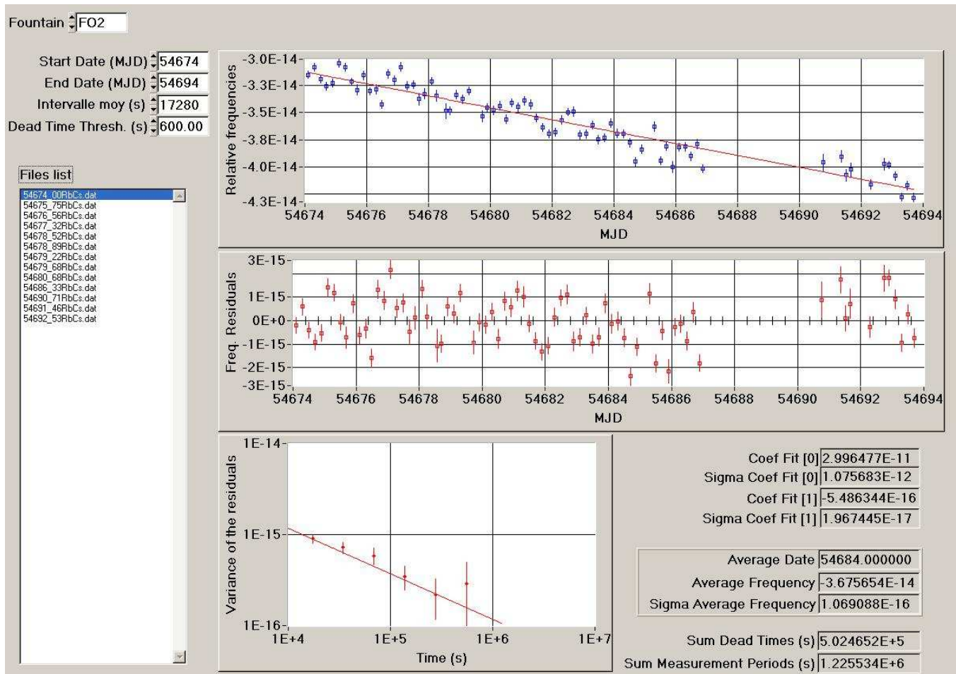
Figure 1: Processing of the data HMaser_{140\ 0890}\text{-FO2} for the period MJD 54674-54694
