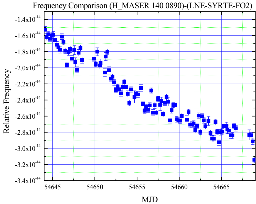
Figure 1: Frequency calibration of Maser 140 0890 by FO2 Fountain between MJD 54644-54669
