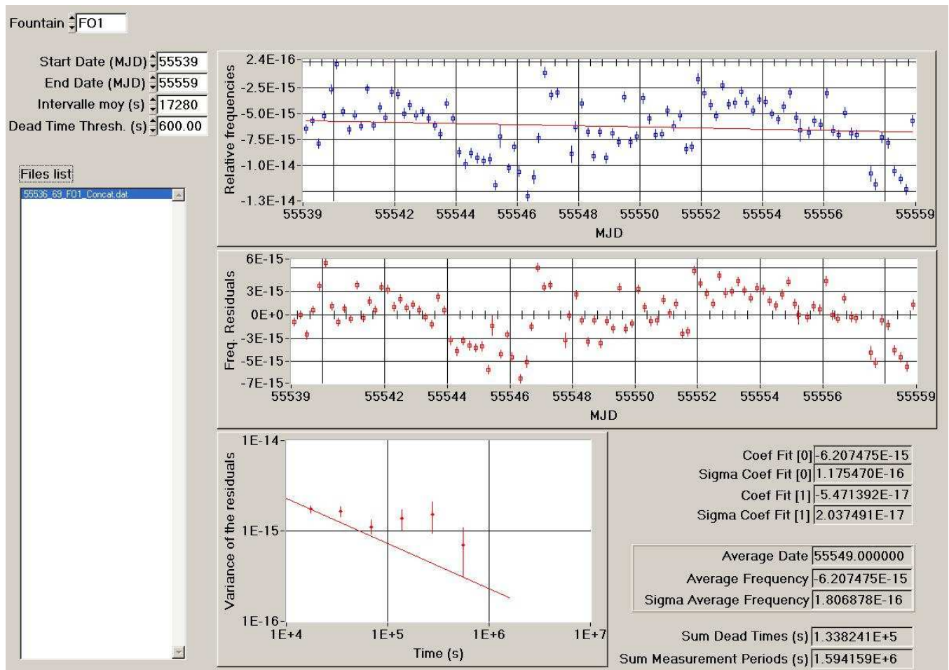
Figure 1: Data processing for the period MJD 55539-55559
