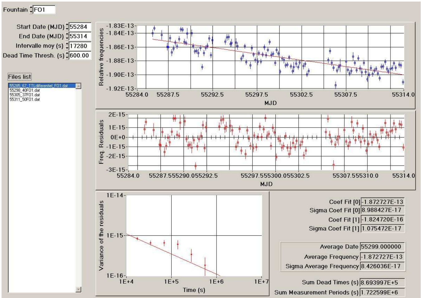
Figure 1: Data processing for the period MJD 55284-55314
