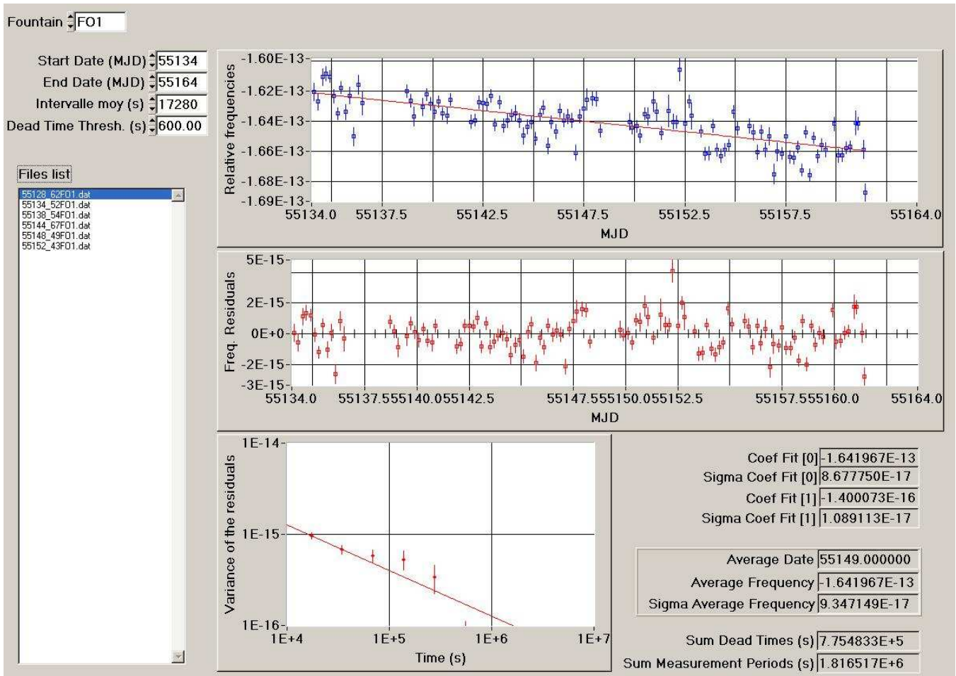
Figure 1: Data processing for the period MJD 55134-55164
