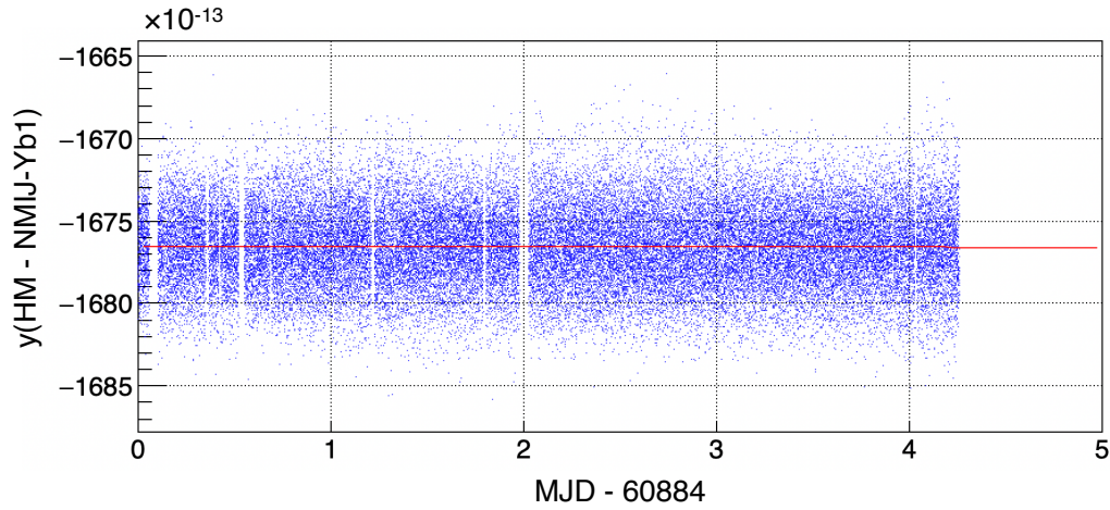
Figure 1. Data points of y(\text{HM} - \text{NMIJ-Yb1}) averaged over 6.8 s. The red line indicates the linear fit used to obtain the drift rate of HM (typically -1 \times 10^{-16}/\text{d} ).
