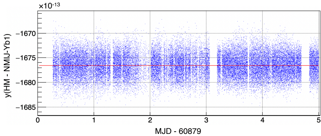
Figure 1. Data points of y(\text{HM} - \text{NMIJ-Yb1}) averaged over 6.8 s. The red line indicates the linear fit used to obtain the drift rate of HM (typically -1 \times 10^{-16}/\text{d} ).
