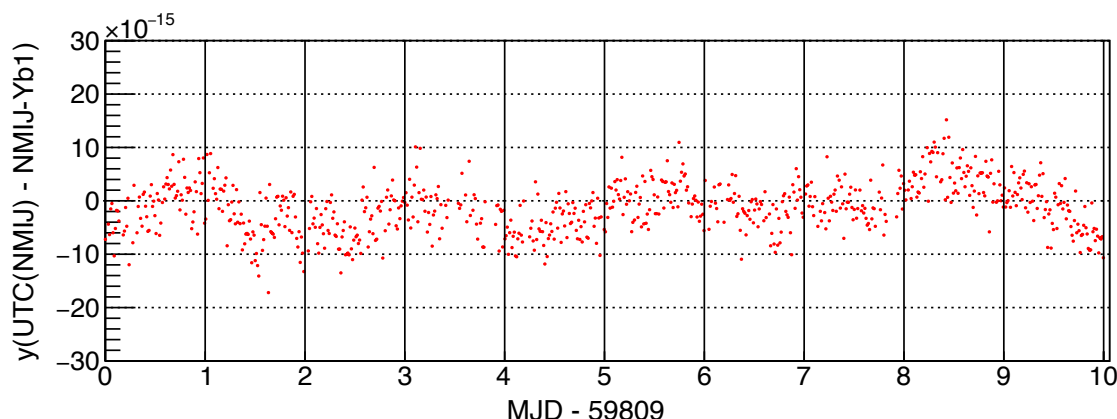
Figure 1. Data points of y(\text{UTC}(\text{NMIJ}) - \text{NMIJ-Yb1}) averaged over 10^3 s.
