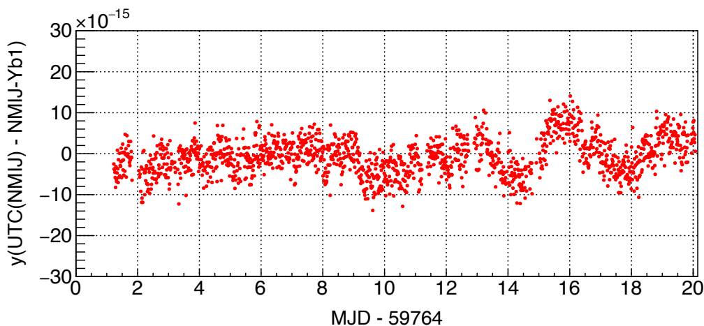
Figure 1. Data points of y(\text{UTC}(\text{NMIJ}) - \text{NMIJ-Yb1}) averaged over 10^3 s.
