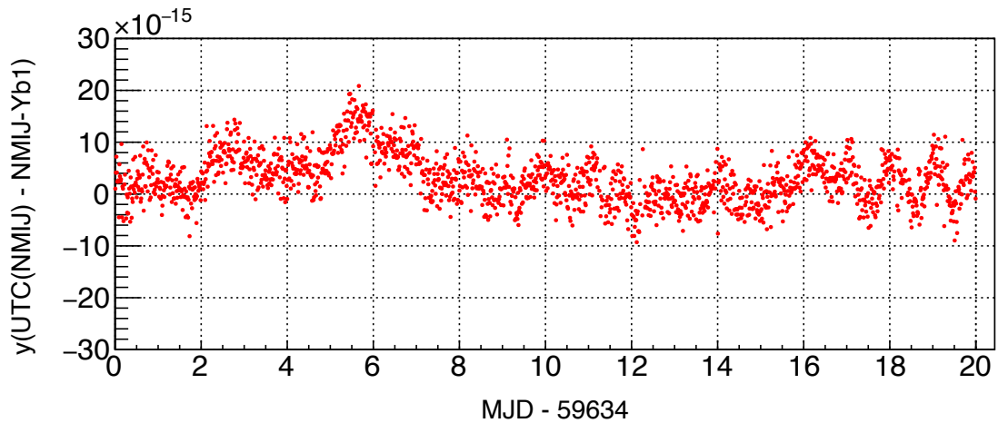
Figure 1. Data points of y(\text{UTC}(\text{NMIJ}) - \text{NMIJ-Yb1}) averaged over 10^3 s.
