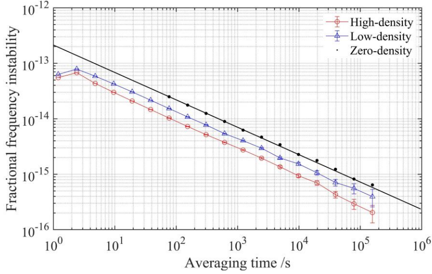
Figure 1. Allan deviation of the relative frequency measured by NIM6 against H-maser 1404821. The data correspond to 22 effective days between MJD 61139 and MJD 61159. The symbols hollow circle, hollow triangle, and solid circle respectively represent the instabilities of frequency at high atom density, at low atom density, and extrapolated to zero density. The solid black line represents the fit for the extrapolated frequency at zero atom density.
