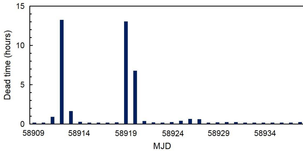
Figure 1 Dead time distributions in Mar., 2020 report period.
