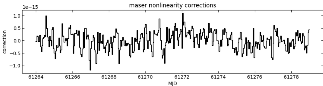
Fig.5. Corrections applied to the assumed frequency of HM 1402014 based on its difference from the ensemble mean. As a correction for instantaneous HM frequency excursions, the overall mean is set to be zero.
