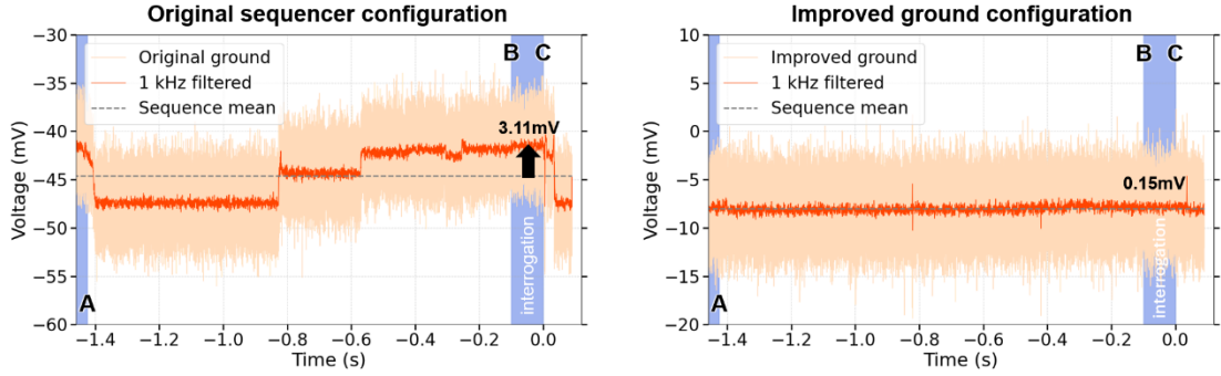
Fig. 1. Electrical measurements: Sampled voltages on the ground signal of a coaxial cable connected to the clock’s sequencer and control systems, measured relative to the ground level of the laser system. ( Left ) With the original electrical configuration of the clock sequencer, the voltage visibly and repeatedly varies with the sequencer’s output state. The voltage measured during the interrogation of the atomic sample (B-C) differs by 3.11 mV from the mean value over the full cycle (A-C). Where such a voltage biases the locking to the reference cavity, the continuous frequency measurement by an optical frequency comb differs from the momentary frequency that the atoms are exposed to. ( Right ) Improved grounding of the sequencer system reduces both the overall ground potential difference and its variation with the output state. The voltage measured during interrogation (B-C) now differs by only 0.15 mV from the full-cycle mean (A-C).
