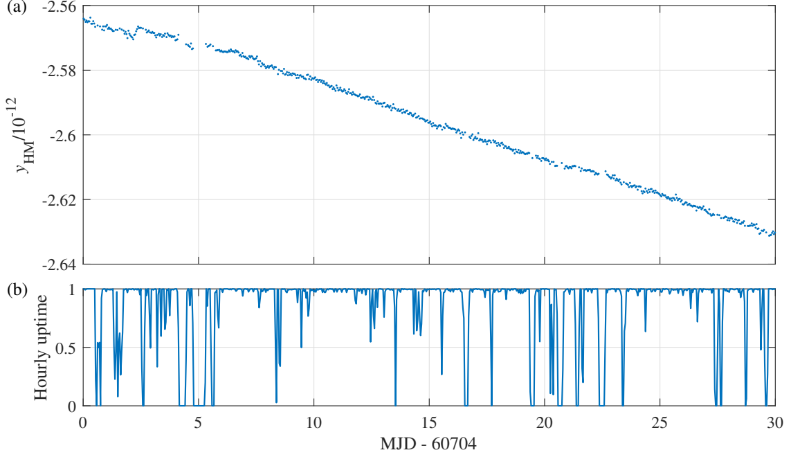
Figure 2: (a) Maser fractional frequency as measured against MIKES-Sr+1 in 3600 s bins and (b) hourly uptime of MIKES-Sr+1 over the evaluation period (total uptime 85.8%).
