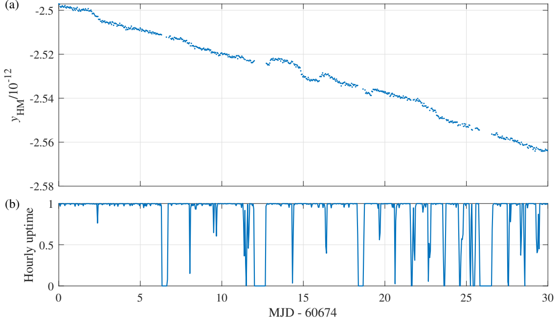
Figure 2: (a) Maser fractional frequency as measured against MIKES-Sr+1 in 3600 s bins and (b) hourly uptime of MIKES-Sr+1 over the evaluation period (total uptime 86.8%).
