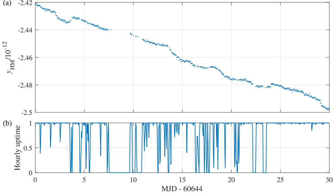
Figure 2: (a) Maser fractional frequency as measured against MIKES-Sr+1 in 3600 s bins and (b) hourly uptime of MIKES-Sr+1 over the evaluation period (total uptime 78.9%).
