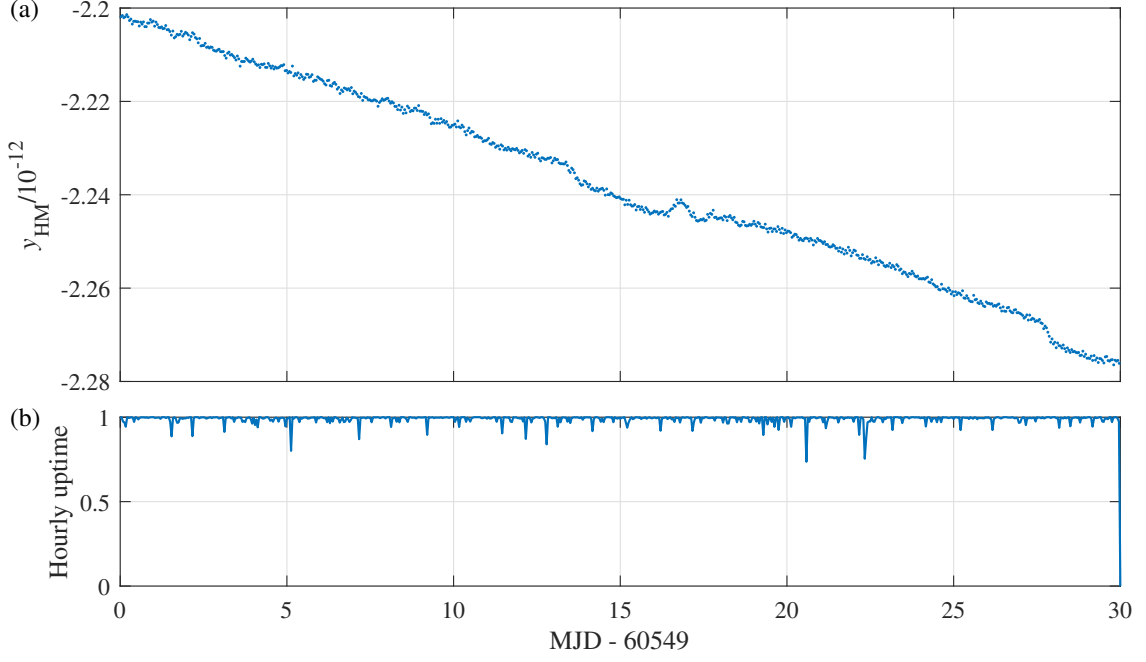
Figure 2: (a) Maser fractional frequency as measured against MIKES-Sr+1 in 3600 s bins and (b) hourly uptime of MIKES-Sr+1 over the evaluation period (total uptime 98.9%).
