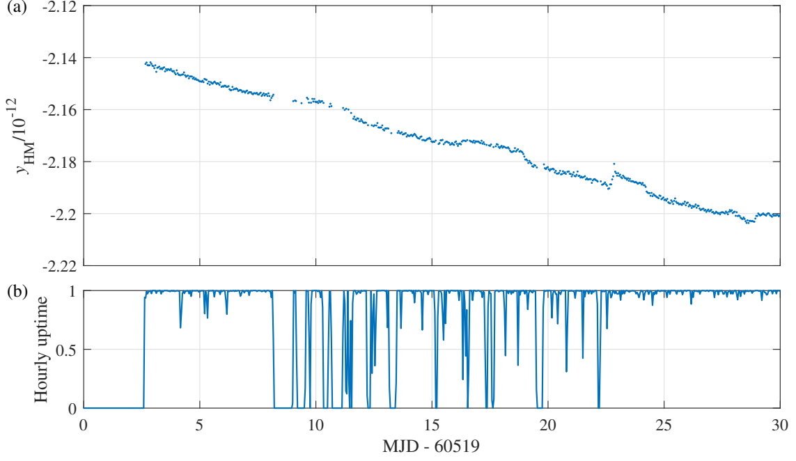
Figure 2: (a) Maser fractional frequency as measured against MIKES-Sr+1 in 3600 s bins and (b) hourly uptime of MIKES-Sr+1 over the evaluation period (total uptime 77.4%).
