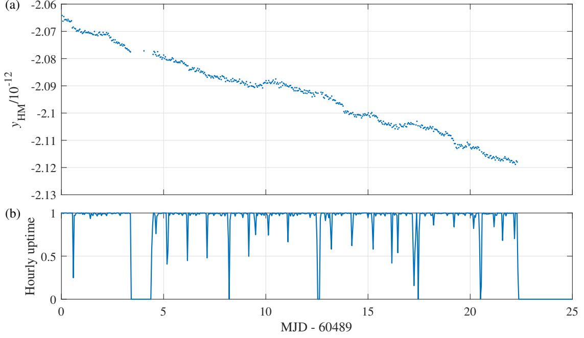
Figure 2: (a) Maser fractional frequency as measured against MIKES-Sr+1 in 3600 s bins and (b) hourly uptime of MIKES-Sr+1 over the evaluation period (total uptime 67.9%).
