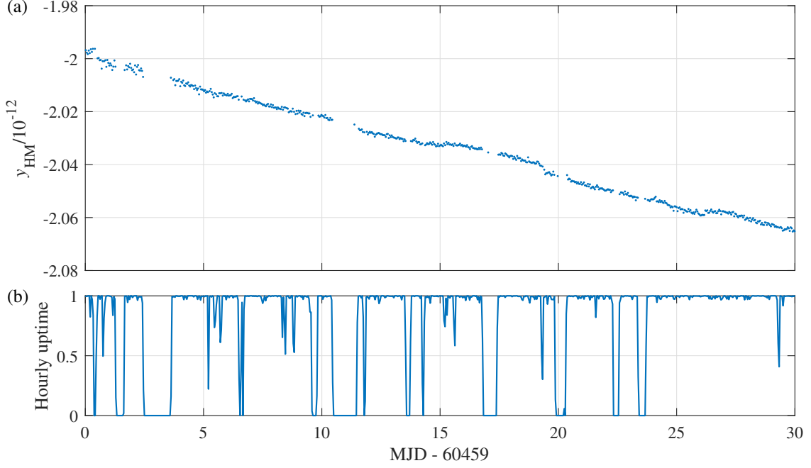
Figure 2: (a) Maser fractional frequency as measured against MIKES-Sr+1 in 3600 s bins and (b) hourly uptime of MIKES-Sr+1 over the evaluation period (total uptime 81.1%).
