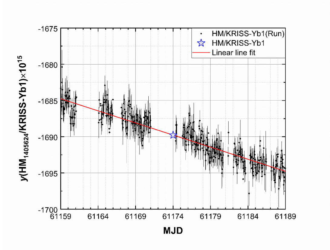
Figure 2. The black points are averaged data of y(\text{HM}_{1405624}/\text{KRISS-Yb1}) over around 3,600 s or less operation time with each uncertainty. The blue star indicates the determined value of y(\text{HM}_{1405624}/\text{KRISS-Yb1}) . The red line is the linear fit (drift rate : -0.334 \times 10^{-15}/\text{d} ) using data from MJD 61159 to MJD 61189 .
