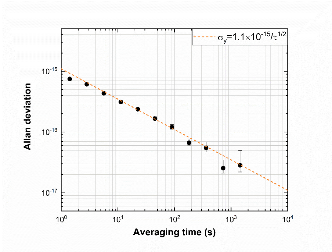
Figure 3. Stability of KRISS-Yb1 in terms of overlapping Allan deviation of the frequency difference between the two interleaved measurements.
