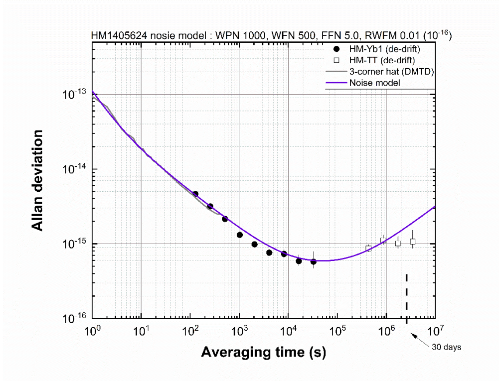
Figure 1. Frequency instability of the hydrogen maser (HM1405624)
