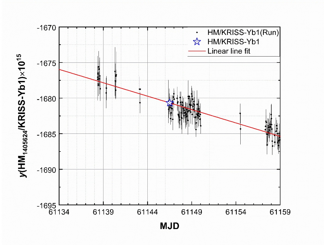
Figure 2. The black points are averaged data of y(HM_{1405624}/KRISS-Yb1) over around 3,600 s or less operation time with each uncertainty. The blue star indicates the determined value of y(HM_{1405624}/KRISS-Yb1) . The red line is the linear fit (drift rate : -0.376 \times 10^{-15}/d ) using data from MJD 61134 to MJD 61159.
